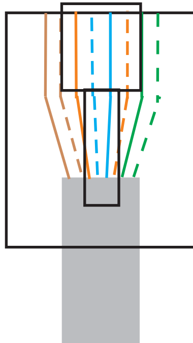
Looking at top view of RJ-45 Male connector
